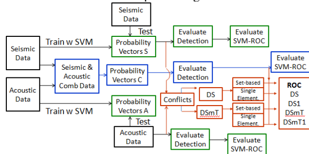
Figure 3. Experimentation Flow.
