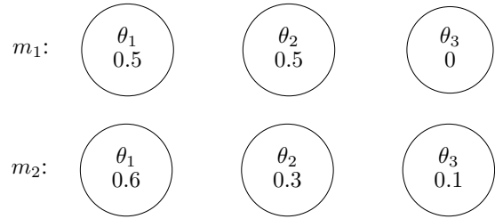
Figure 1. Bayesian bba's
