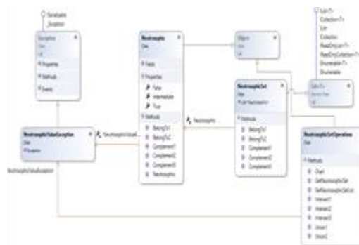
We introduce the neutrosophic package class diagram :
