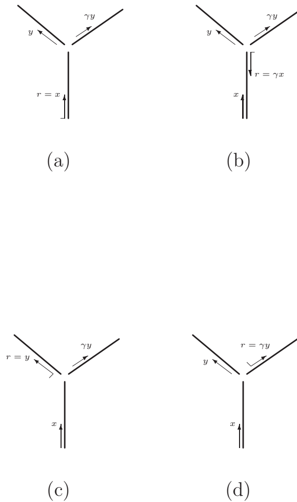
Fig.8.1 Rootings in Example 1
