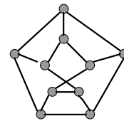
C_{15,3}
