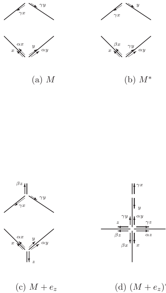
Fig.3.10 Duality between appending and splitting an edge
