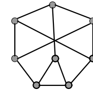
C_{12,2}
