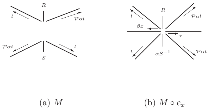
Fig.3.9 t and l transitive
