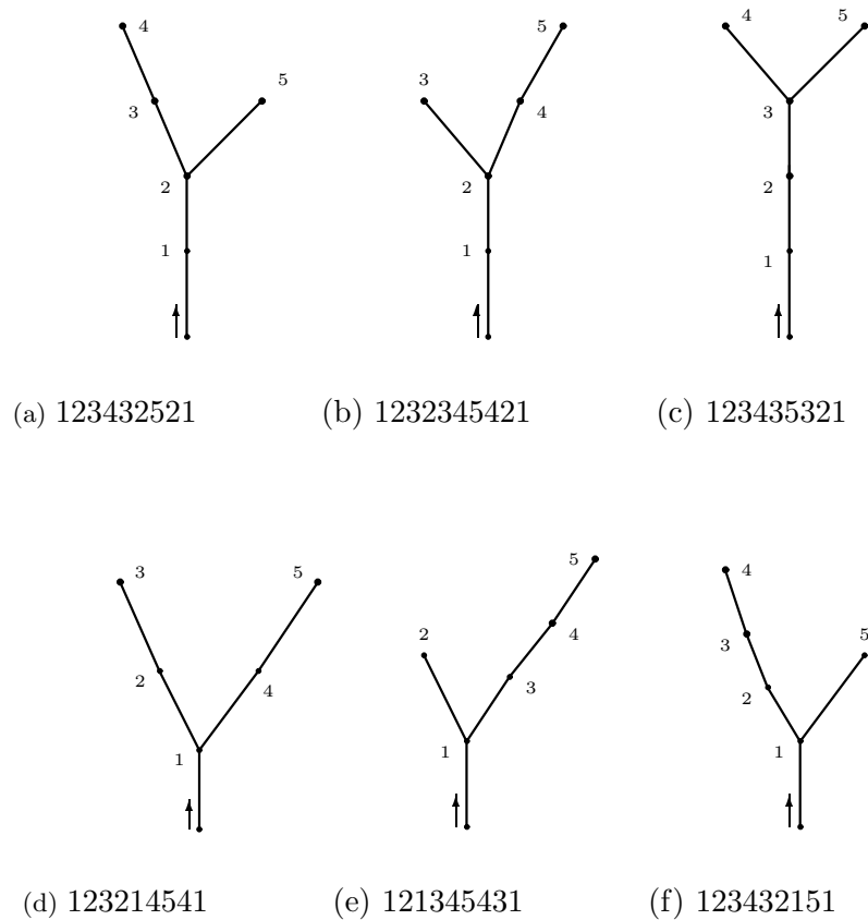
Fig.13.3 Trees with \underline{n} = (2, 2, 1)
