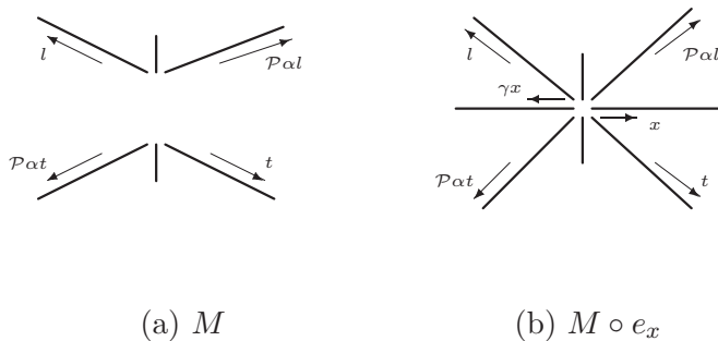
Fig.3.8 t and l nontransitive
