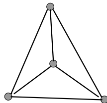
C_{6,1}
