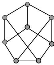
C_{12,3}
