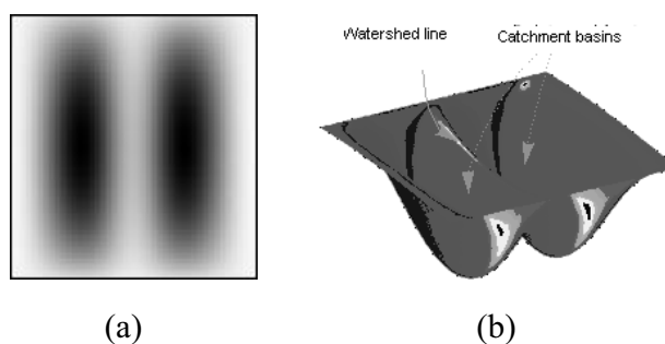
Figure 2.1. Watershed concept. (a) Two dark blobs. (b) 3D view of the watershed image of (a).
