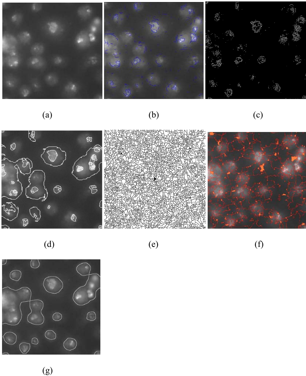
Figure 2.11. Cloud image. (a) Original image. (b) Result using the embedded confidence method. (c) Result using the Sobel operator. (d) Result using the mean-shift method. (e) Result using the watershed in Matlab. (f) Result using toboggan-based watershed. (g) Result using the proposed method.
