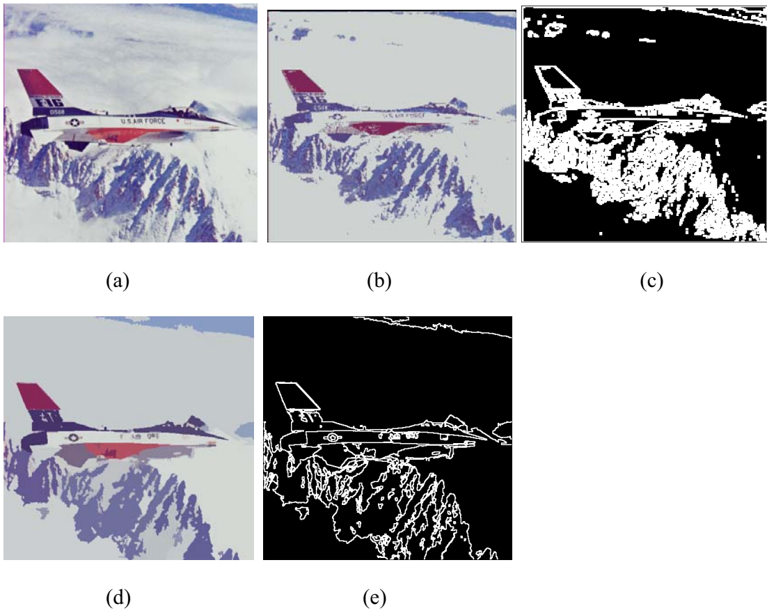
Figure 4.8. Plane image (469x512): (a) Original image. (b) Result by applying fuzzy homogeneity. (c) Boundaries of (b). (d) Segmentation result of the proposed method ( \lambda = 0.04 ). (e) Boundaries of (d).
