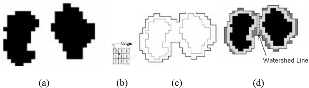
Figure 2.9. Watershed method. (a) Two regions that have value 0. (b) 3 \times 3 structure element (c) Dilation of the two regions. (d) Dam construction.
