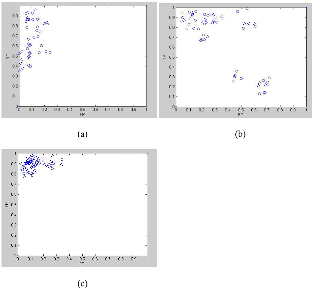
Figure 3.11. TP versus FP plotting. (a) Plotting of activate contour method. (b) Plotting of TE method. (c) Plotting of proposed method.
