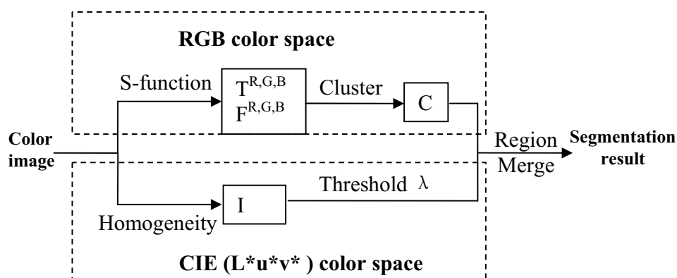
Figure 4.3. Flowchart of proposed method.
