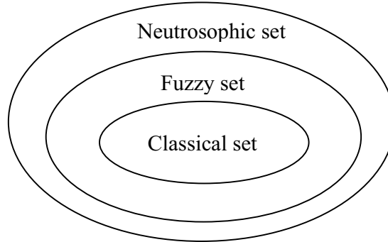
Figure 1.1. Relationships among neutrosophic set and other sets.
