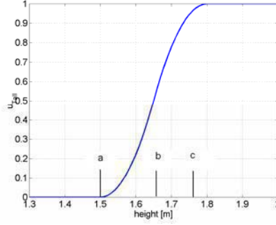
Figure 2.3. S-function.
