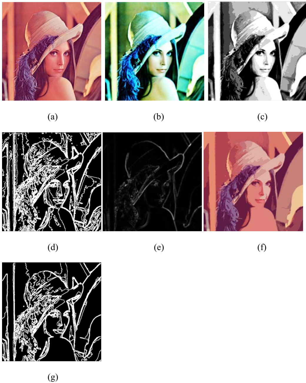
Figure 4.4. Steps of proposed algorithm: (a) 512x512 Lena color image. (b) Result after applying the S-function and enhancement. (c) Clusters result in T . (d) Boundaries based on (c). (e) Indeterminacy value image in I . (f) Final result of the proposed segmentation method ( \lambda = 0.04 ). (g) Boundaries of (f).
