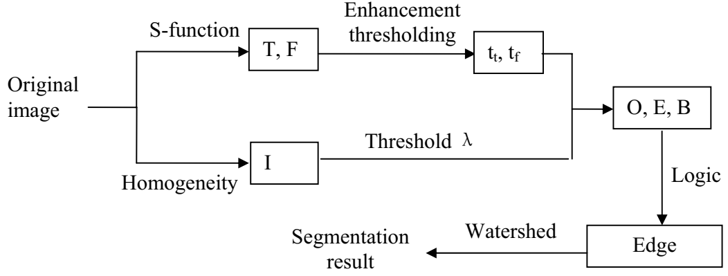
Figure 2.2. Flowchart of proposed method.
