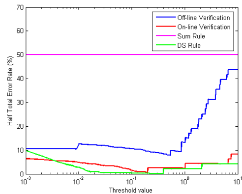
Figure 5. HTER Curves of Off-line, On-line and Combined Systems for Signature Verification
