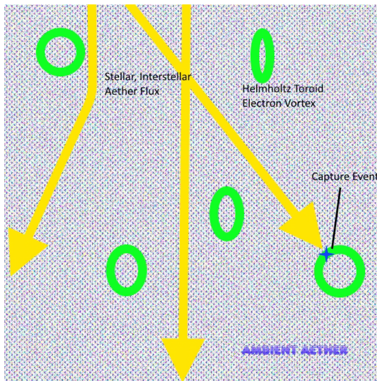
Figure 2. electron vortex capture event (after R.N. Boyd)
