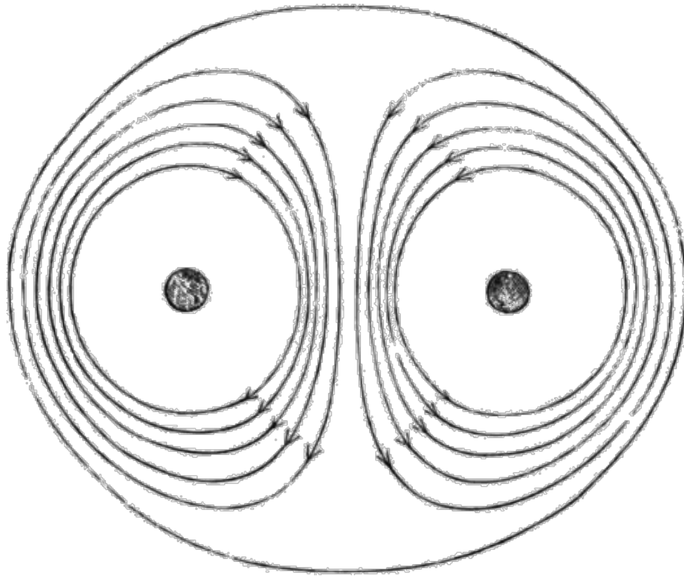
Figure 4. Helmholtz's atom model should be applied to electron vortex (after RN Boyd)
