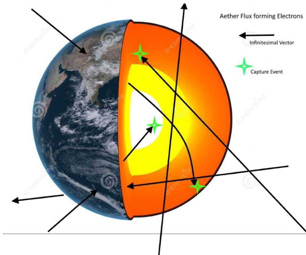
Figure 3. Illustration on how matter creation can take place in inner core of Earth
