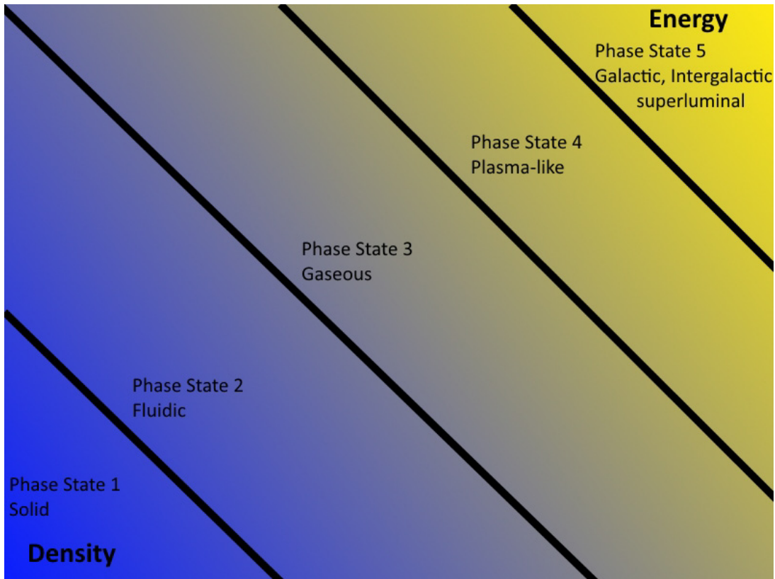
Figure 5. Mishin's 5-phase aetherdynamics .
