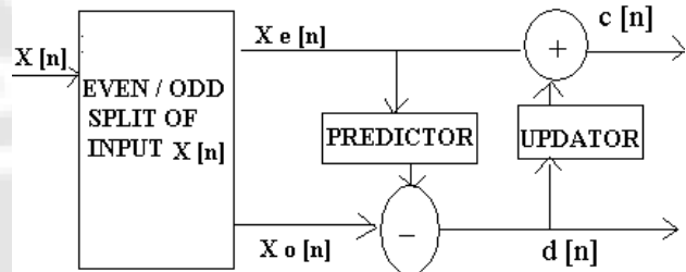
Figure 2: Lifting Scheme
