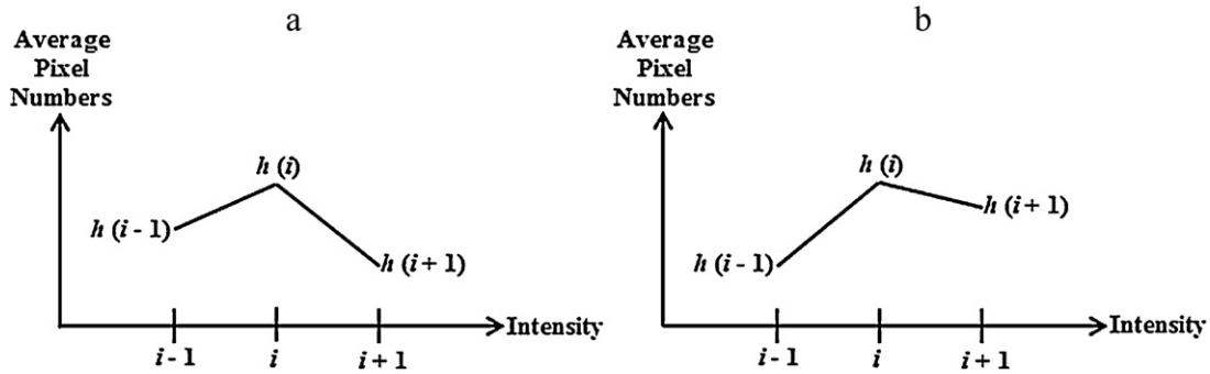
Fig. 2. Possible scenario for intensity level i to be identified as peak by Eq. (8), (a) h(i-1) > h(i+1) and (b) h(i-1) < h(i+1) .
