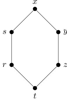
FIGURE 5. C_6 as an (x, t) -friendship graph.
