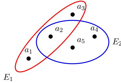
FIGURE 1. An example of hypergraph with 2 hyperedges.
