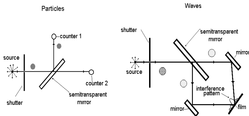
Fig.1. Experiments with individual photons on semitransparent mirror.
