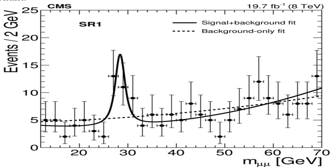
Fig.6. Peak of energy at 28GeV
