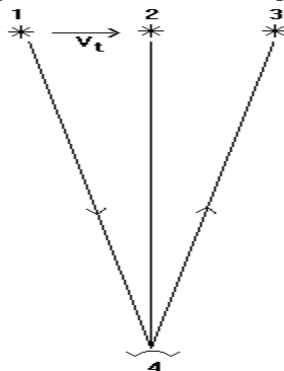
Fig.10. The past (1), verily (2) and the future (3) positions of astronomical object. Portion of light emitted by object in position (1) reaches observer (4) many years after. During this time the object that moves
