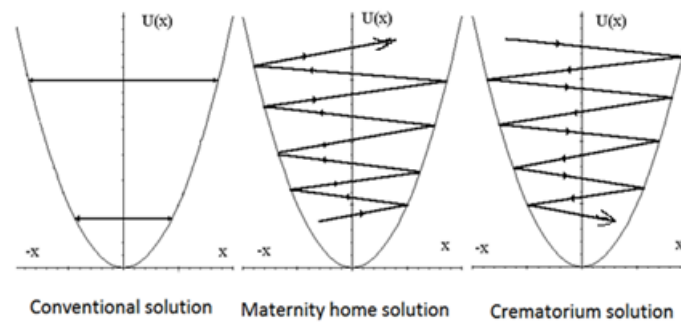
Fig. 7. Solution of UQT for harmonic oscillator
