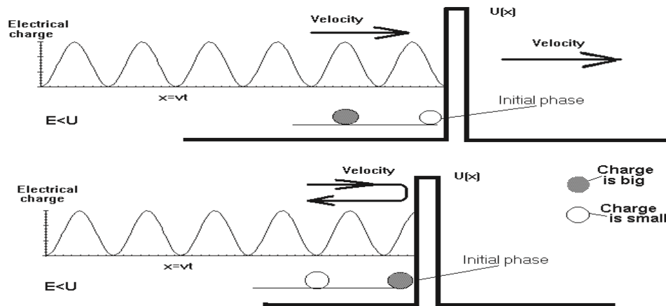
Fig.9. Illustration of the tunnel effect
