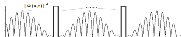
Fig.10. Visual image of particles passing through two potential barriers - scheme of New Maxwell Demon.
