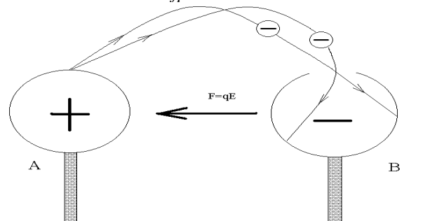
Fig. 8. Work for transferring the charge depends on the mode of transferring and on the path.
