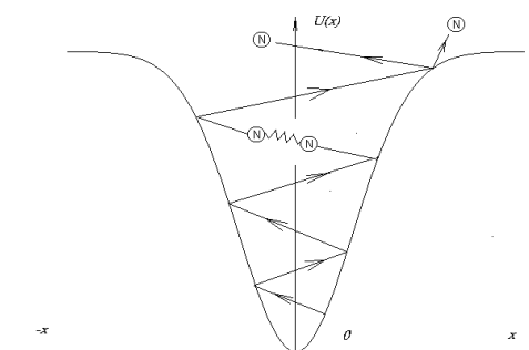
Fig.8. Oscillation of Nitrogen molecule in potential well of catalyst.
