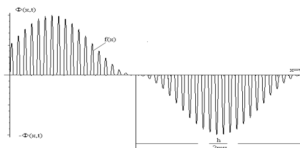
Fig. 2. Behavior of wave packet in linear dispersion medium (i.e., rather like a series of stroboscopic photographs).
