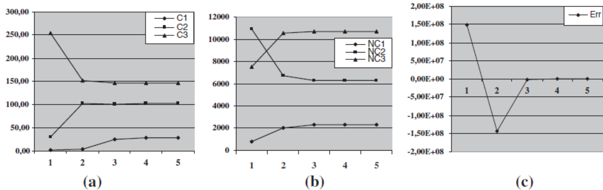
Figure 5: Dynamic changes of the different classification parameters starting from the class centers (c_1, c_2, c_3) = (1, 30, 255) .
