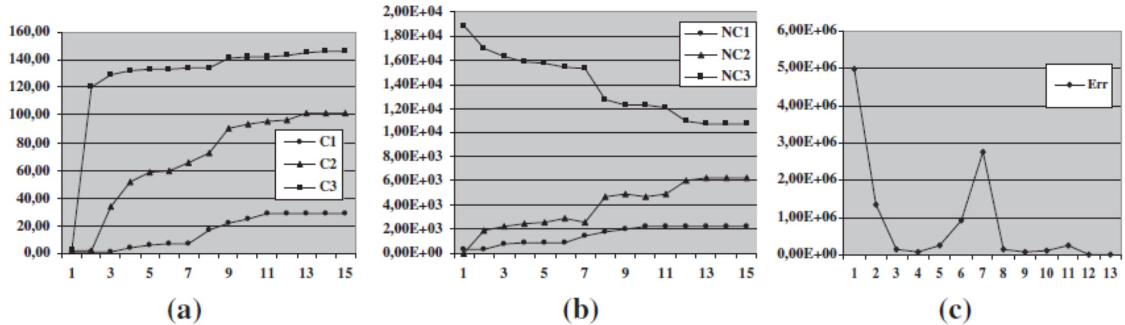
Figure 4: Dynamic changes of the different classification parameters starting from class centers (c_1, c_2, c_3) = (1, 2, 3) . (a) class centers, (b) cardinality of each class, and (c) absolute value of error of the objective function.
