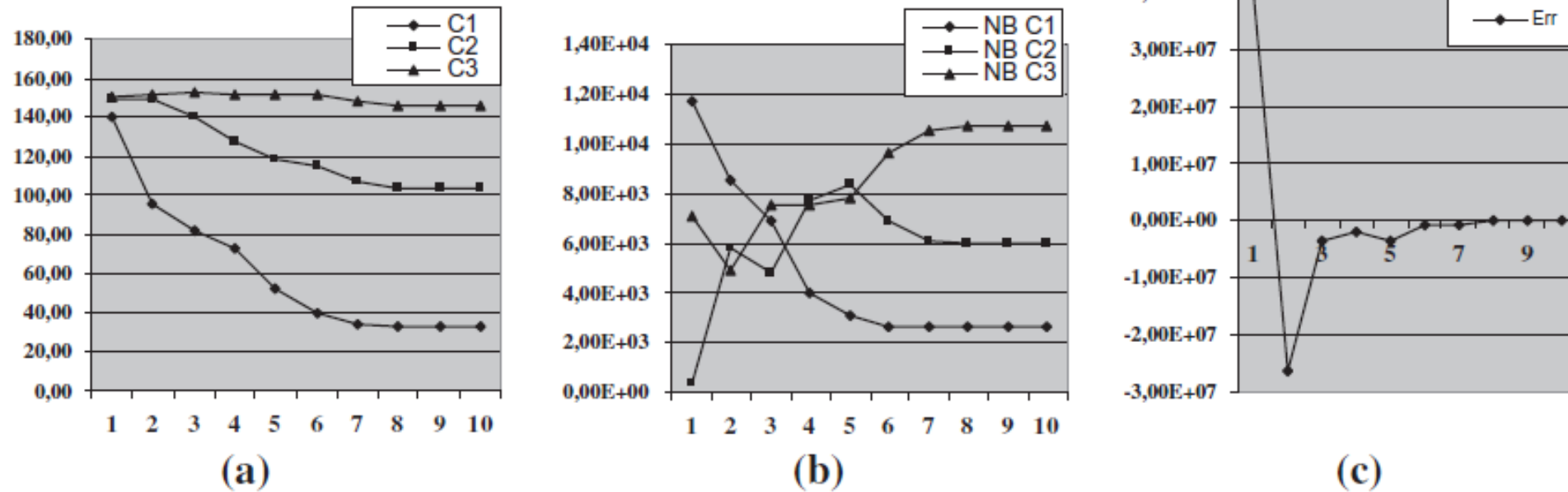
Figure 6: Dynamic changes of the different classification parameters starting from class centers (c_1, c_2, c_3) = (140, 149, 150) .
