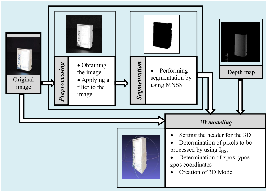
Fig. 8. 3D modeling system flow diagram.
