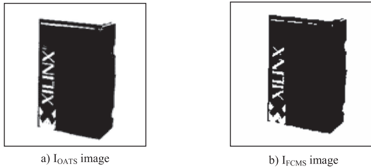
Fig. 7. Segmentation images.
