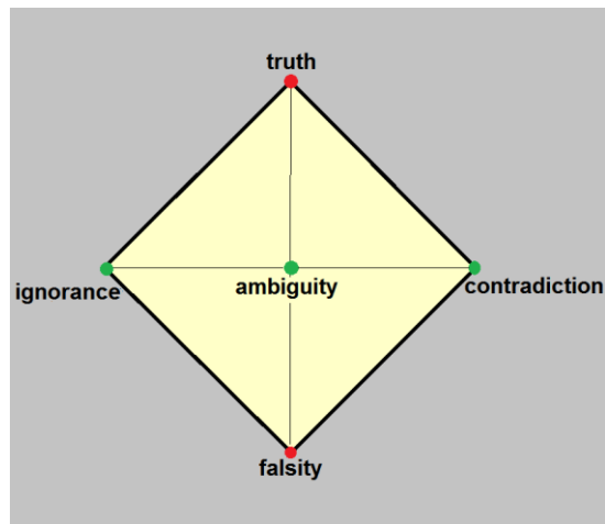
Fig. 4. The bottom square of the neutrosophic cube.
