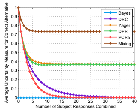
(f) Average uncertainty for true alternative after fusion, "Intersubject Conflict Discounting" operator input construction case
