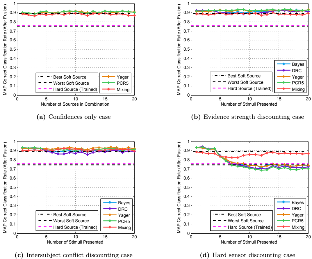
Figure 6.10: Estimated post combination correct classification rate using a maximum a posteriori (MAP) decision rule versus the number of stimuli presented to the hard and soft sources when training the RDM hard sensor online. The different lines represent the fusion operators being investigated. In all simulation cases, the hard sensor was the first source in the combination, followed by a random permutation of five soft sources. Results averaged over 10,000 simulation trials. MAP correct classification rates of the best and worst soft sources and the trained hard source are shown for comparison.
