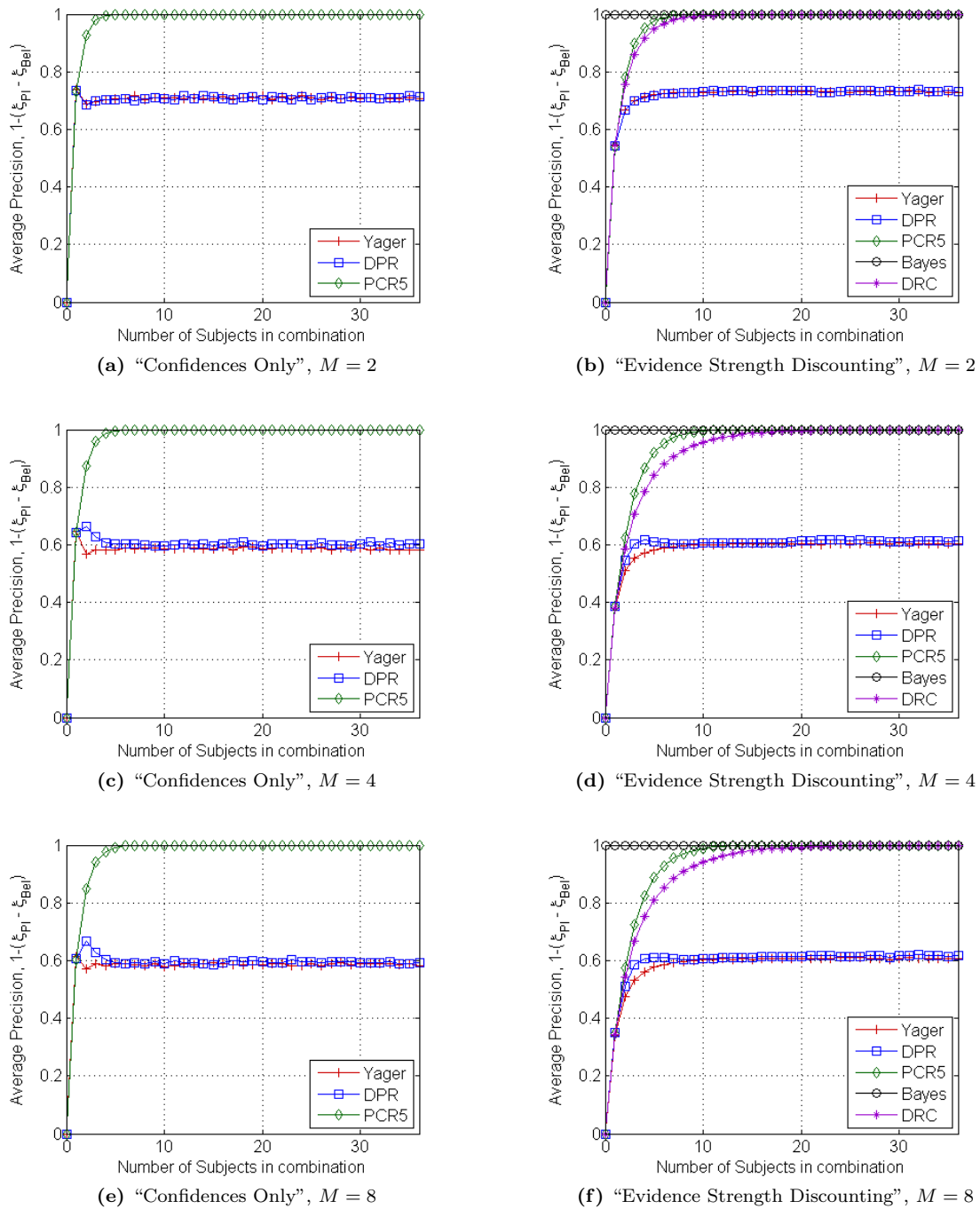
Figure 5.13: Average precision performance ( i.e. , 1 - (\xi_{P1} - \xi_{Bel}) ) for each of the five fusion methods versus the number of sources present in combination (higher is better). Results simulated over 10,000 trials for the M-ary line length discrimination task with M = 2, 4, 8 .
