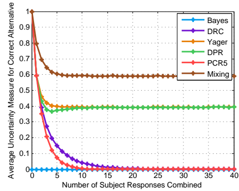
(d) Average uncertainty for true alternative after fusion, "Evidence Strength Discounting" operator input construction case
