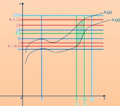
Example for the Neutrosophic Intermediate Value Theorem
