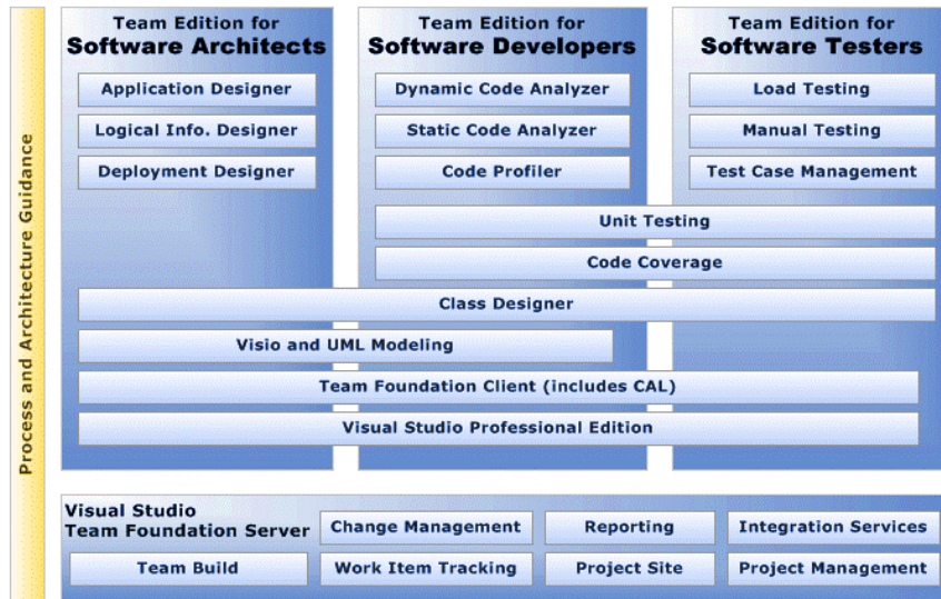
Figure 3. Visual Studio Team Suite as a support tool
