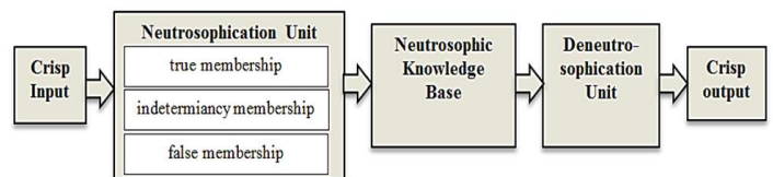
Figure 3: Block Diagram of Neutrosophic Inference System
