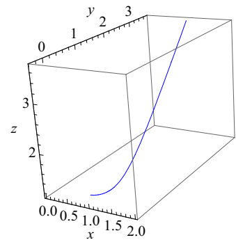
Fig. 6 From left to right, the e_1e_2 , e_1e_3 and e_1e_2e_3 Smarandache curves of \delta .
