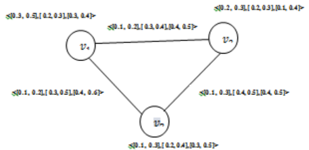
Fig. 2. Interval valued neutrosophic graph
