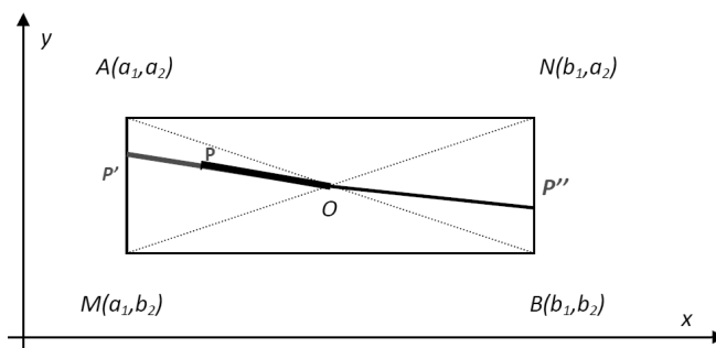
Fig. 3: P is an interior point to the rectangle AMBN and the optimal point O is in the center of symmetry of the rectangle.
