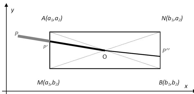
Fig. 4: P is an exterior point to the rectangle AMBN and the optimal point O is in the center of symmetry of the rectangle.
