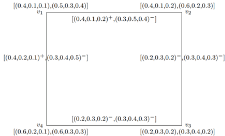
Figure-3.1: Interval valued signed neutrosophic graph
