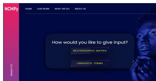
Figure 6: Option Selection
