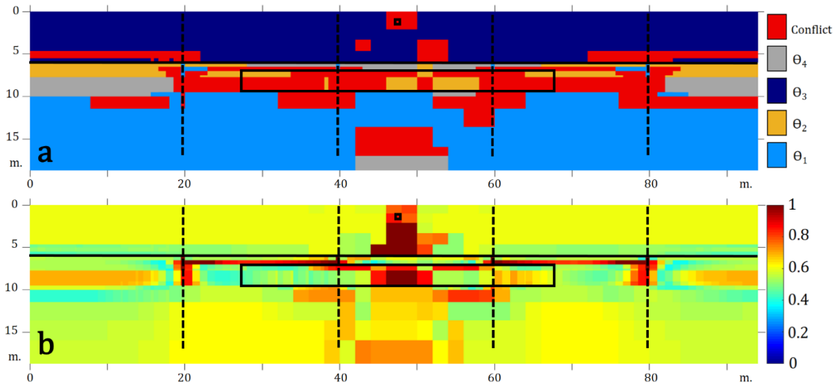
Figure 2 Data merging with Smets' combination rule: b ) represents the BBAs associated to the most plausible events presented in a ). The black lines stand for the interfaces and the conductive anomaly fixed in the ER model (Figure 1.a) while the dashed lines stand for the boreholes position.
