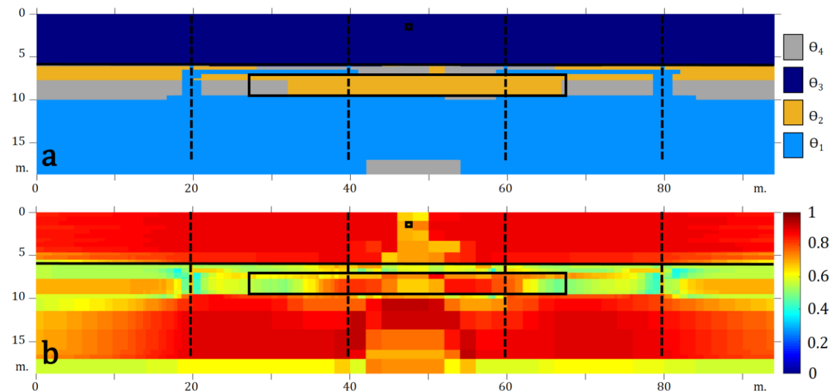
Figure 3 Data merging with PCR5 normalization rule: b ) represents the BBAs associated to the most plausible events presented in a ). The black lines stand for the interfaces and the conductive anomaly fixed in the ER model (Figure 1.a) while the dashed lines stand for the boreholes position.
