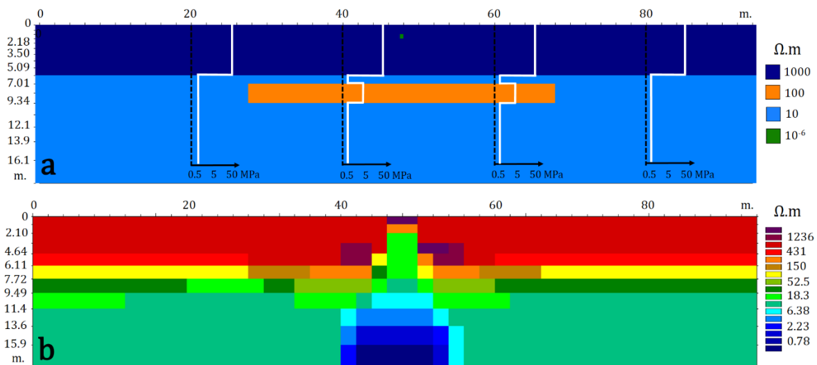
Figure 1 2D section of subsoil displaying a) true ER with boreholes position in dashed line and associated cone bearing values in white and b) inverted ER with model data block.
