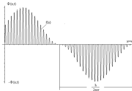
Fig. 2. Behavior of wave packet in linear dispersion medium (i.e., rather like a series of stroboscopic photographs).
