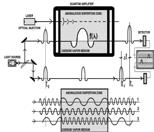
Fig. 5. Experiments of L.Wang - superluminal light propagation. Such experiments were carried out by several teams (in Berkeley, Vienna, Cologne, Florence, etc.) and they emerged the superluminal speeds. The most interesting were investigations [27, 32] in which Lijun Wang found out velocity 310 times higher than the speed of the light (Fig. 5). Wang gave the same interpretation as ours, but only for an impulse of light. In this case it was a wrong interpretation, because in the experiment the envelope of the light pulse was not distorted absolutely (obligatory condition), and Wang noticed that amazing fact. He supposed that the special theory of relativity was absolutely destroyed. But it was not quite true. Our idea that particles are wave packets is an absolutely original idea for the worldwide science. The waves at the Fig. 5 have to be realized as separated partial waves of the spectral decomposition of the wave packets of the separated photons, but not as a spectral decomposition of the light pulse. Then the form of the momentum envelope will not be distorted.
