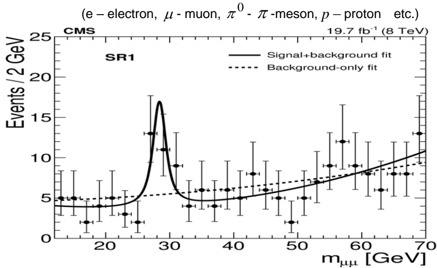
Fig.6. Peak of energy at 28GeV
